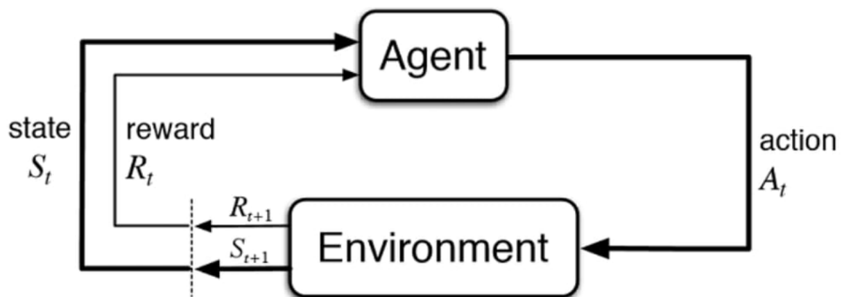
Figure 2. Reinforcement Learning
