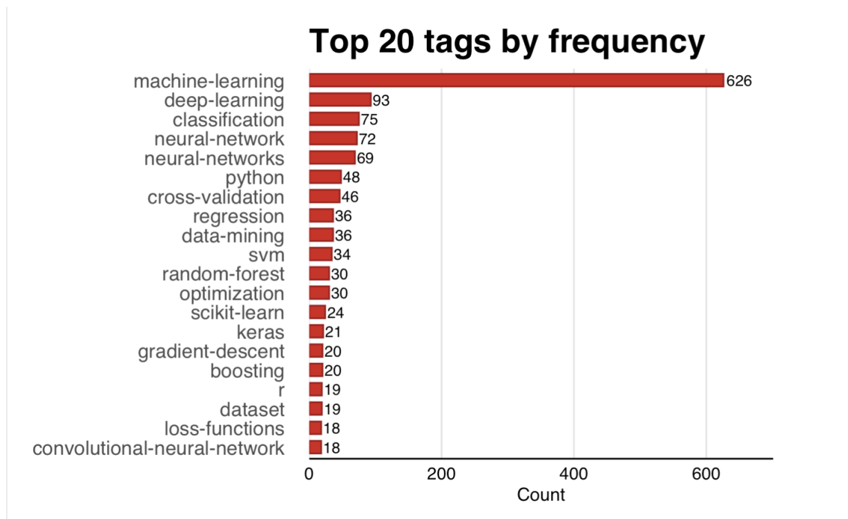
Figure 5. Top 20 tags by frequency. machine-learning dominates with 626 occurrences, followed by deep-learning (93) and classification (75).
